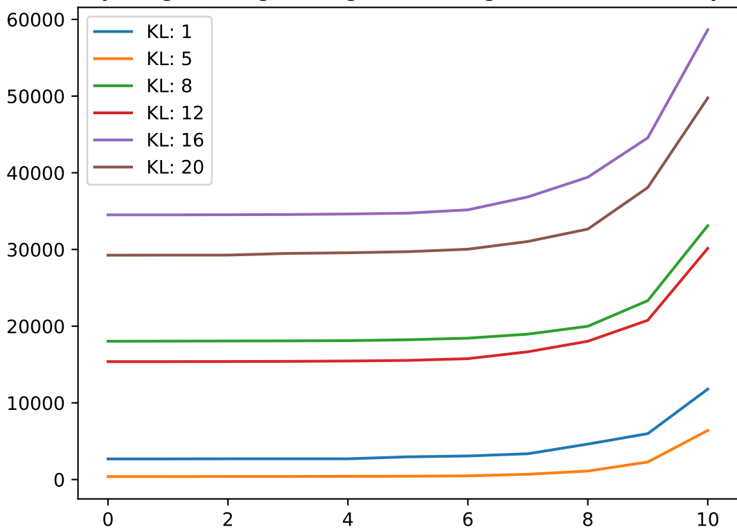
Memory usage of LogisticRegression for gaussian data of varying KL
